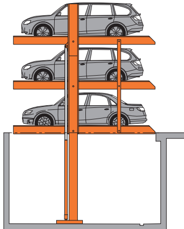
System lifted
