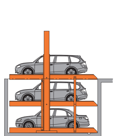
System lowered
